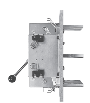
B電源側“入”状態 B power source side “ON”
