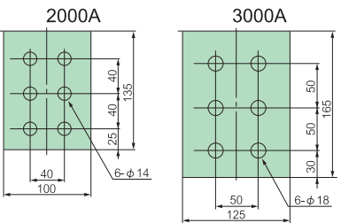
主回路端子詳細 Detail of main circuit terminal
